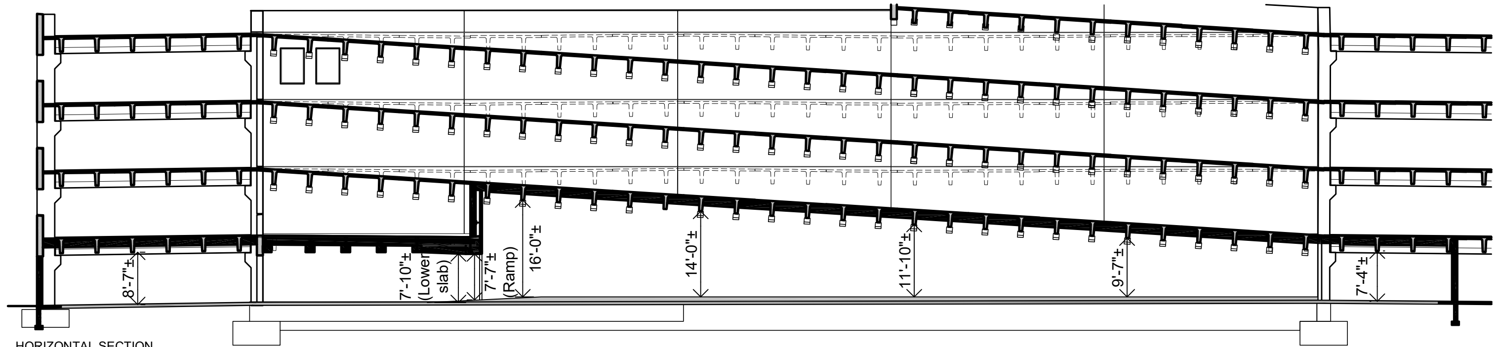
HORIZONTAL SECTION
